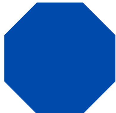
octagon
