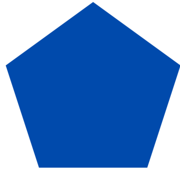
pentagon
