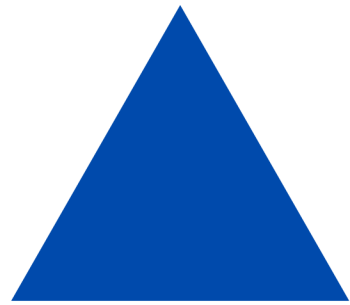
triangle
