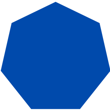
heptagon
