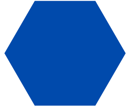
hexagon
