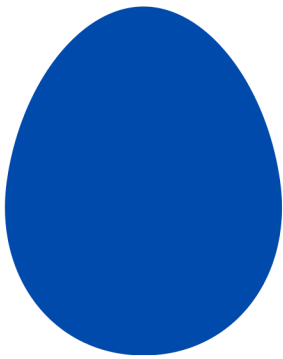
ellipse
