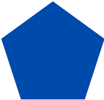
pentagon
