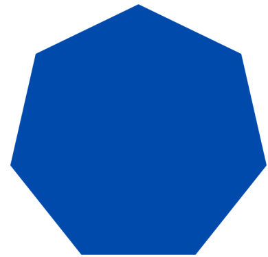
heptagon
