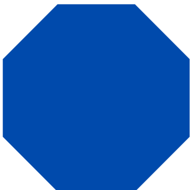
octagon
