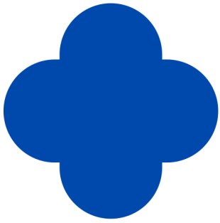
quatrefoil
