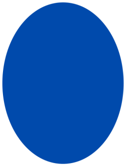
oval
