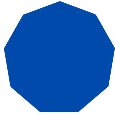
nonagon
