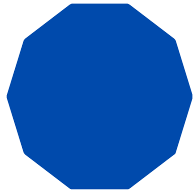
decagon
