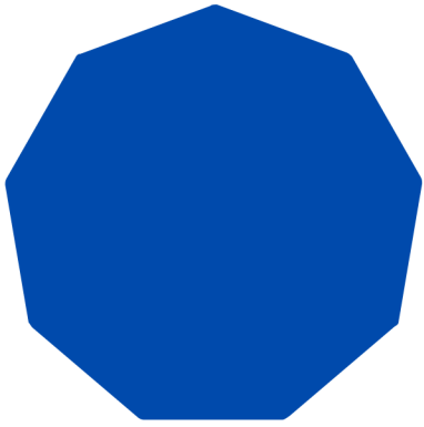
nonagon
